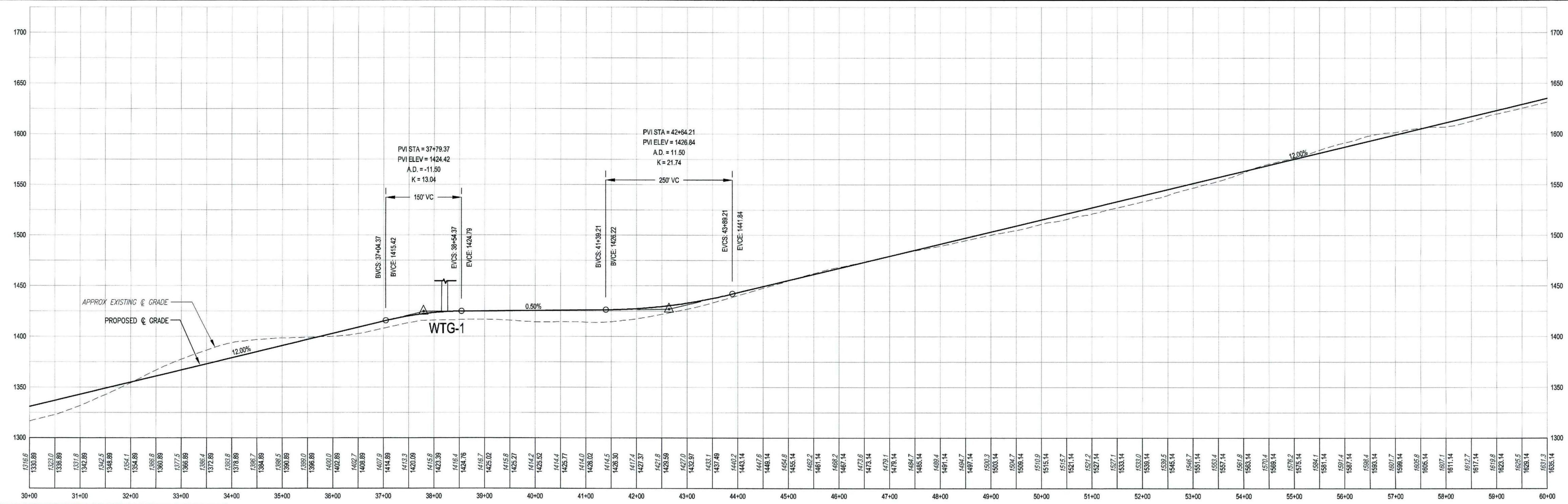
PROFILE: MAIN ACCESS ROAD STA 30+00 TO 60+00 SCALE: HORIZ: 1"=100' VERT: 1"=50'
