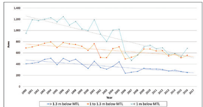
Figure 3 Acres of Eelgrass in Particular Depth Regimes in Great Bay. New Hampshire Department of Environmental Services analysis of loss of eelgrass by depth in Great Bay only. MTL = mean tide.
